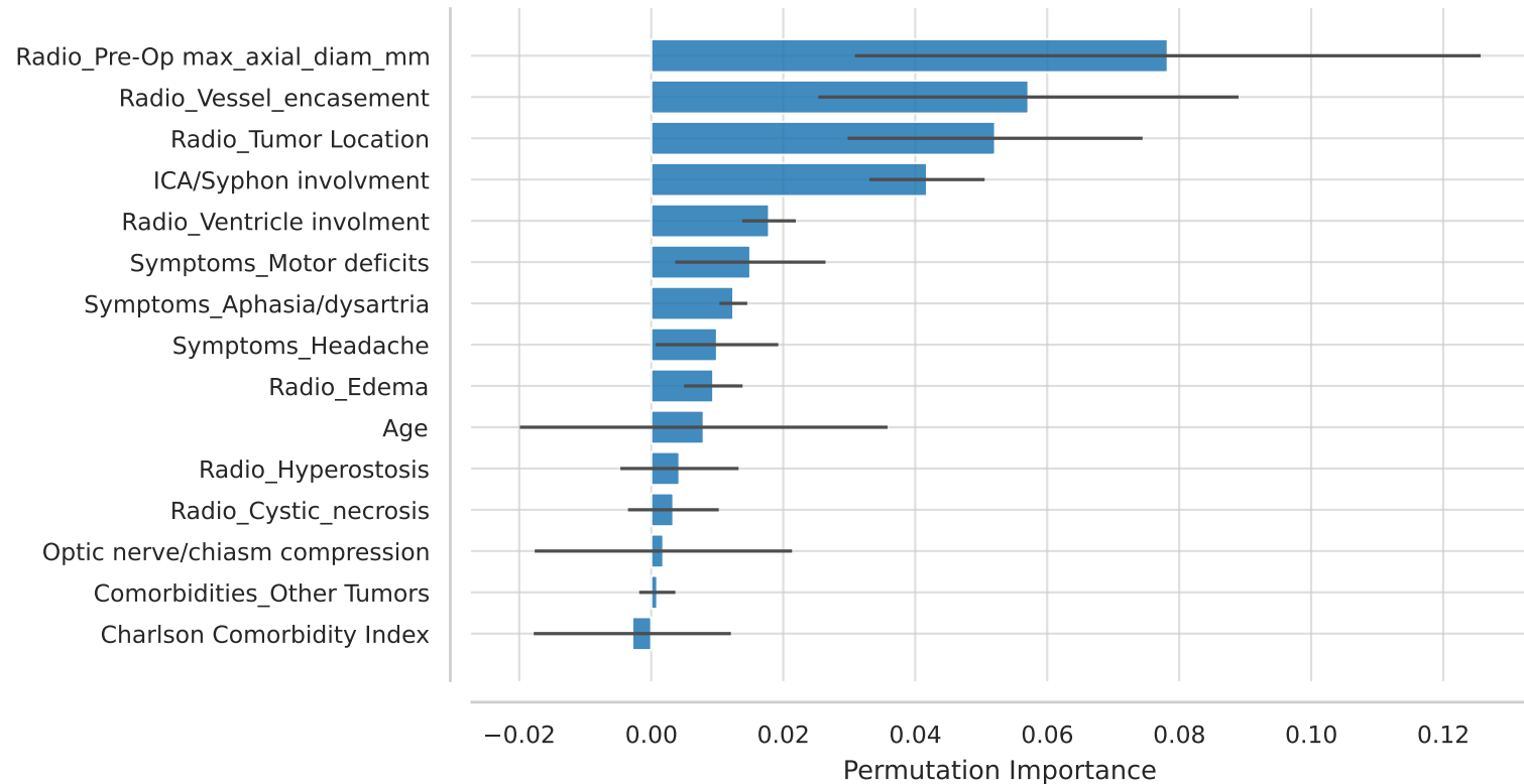
Feature Importance (RF)
